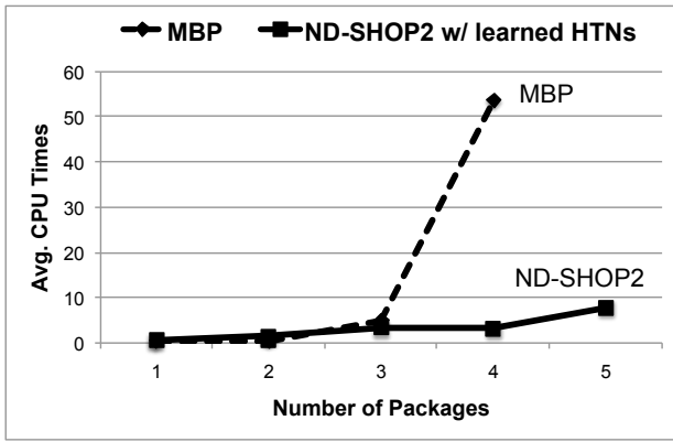
Figure 1: Average running times for ND-SHOP2 using the learned HTNs and MBP, as a function of increasing number of packages in the Robot Navigation domain.
