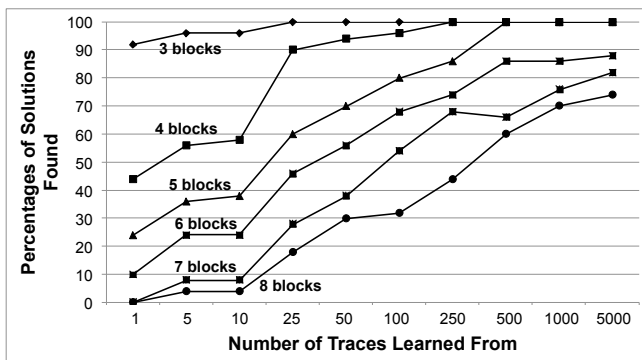
Figure 3: Learning rate for HTN-MAKER ND in the nondeterministic Blocks World domain.
