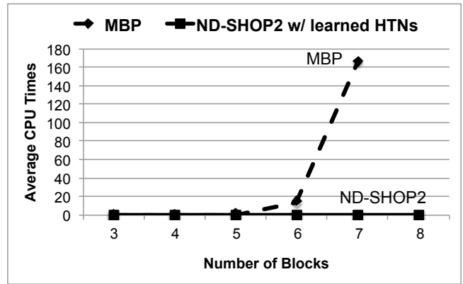
Figure 2: Average running times for ND-SHOP2 using the learned HTNs and MBP, as a function of increasing number of blocks in the nondeterministic Blocks World domain.
